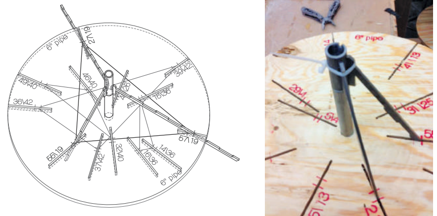
Fig. 6: Steel assembly process: precise horizontal angles registered by angle-finder welding jig. Radially-cut steel pipe, flat-cut steel struts, and plywood angle-finder jig.
